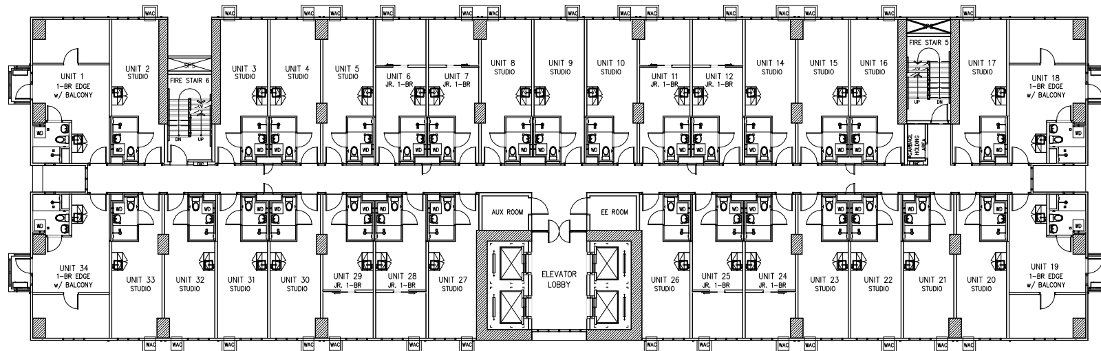
KEY PLAN
